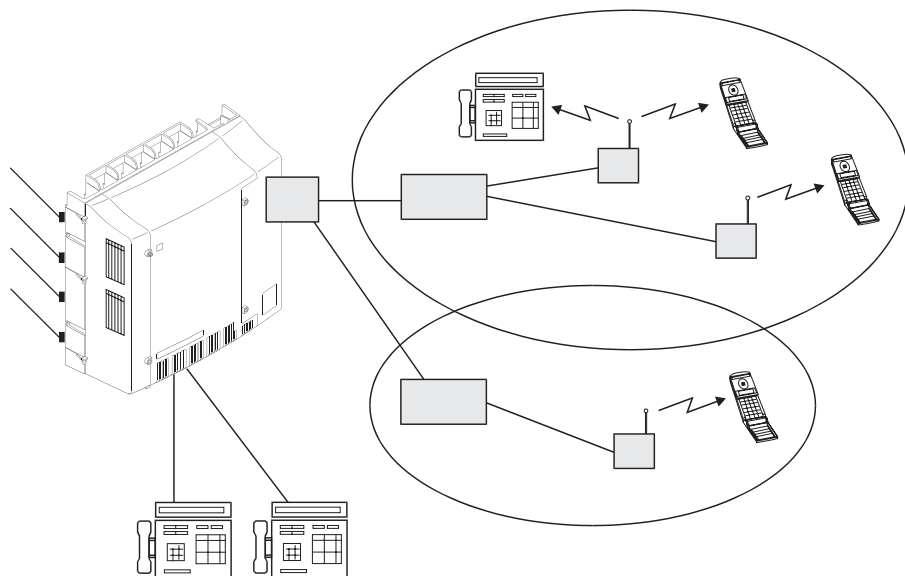
Figure 6-2. Long-Range mobility
